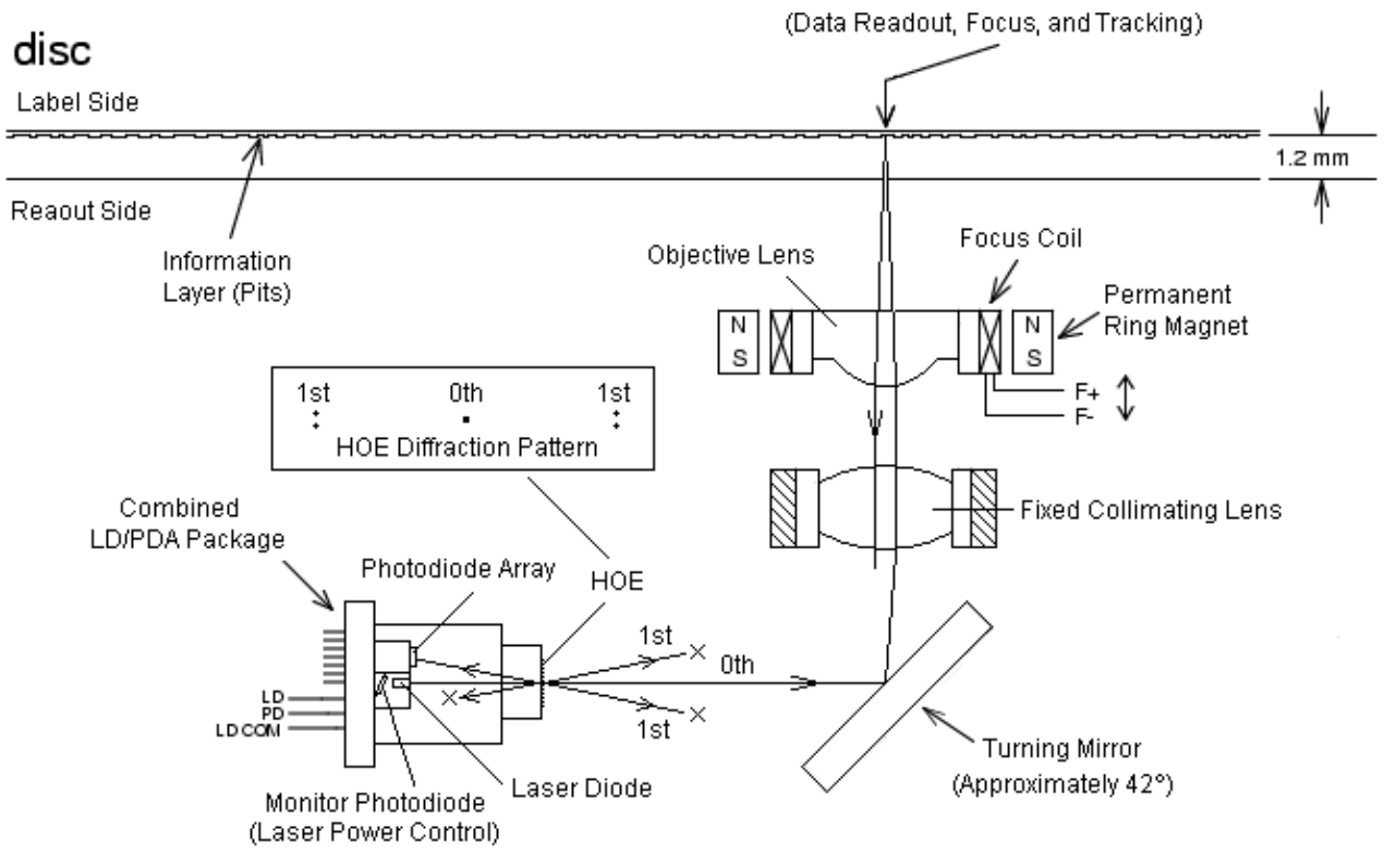
Simple Optical Pickup Organization
